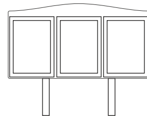
1600mm x 850mm aluminium board - curved or flat top 3 x A2 poster cases 2 x 76mm diameter aluminium posts £855.00 + vat
