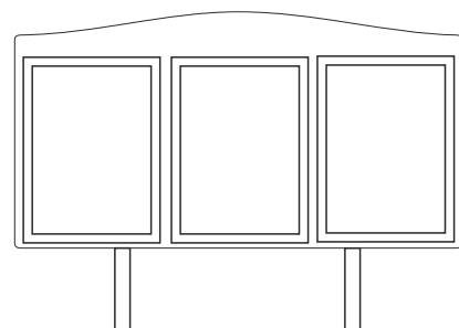
2300mm x 1200mm aluminium board - curved or flat top 3 x A1 poster cases 2 x 76mm diameter aluminium posts £1090.00 + vat
