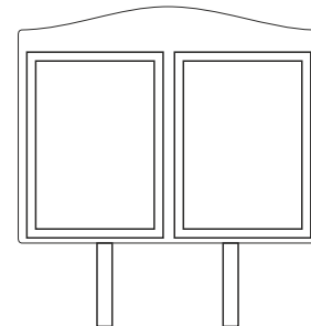
1500mm x 1200mm aluminium board - curved or flat top 2 x A1 poster cases 2 x 76mm diameter aluminium posts £875.00 + vat
